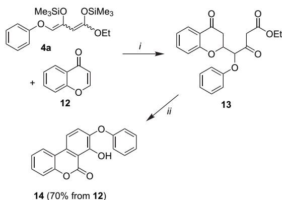
Scheme 6. Synthesis of 14 : (i) (1) \text{Me}_3\text{SiOTf} (0.3 equiv), 20^\circ\text{C} , 1 h; (2) 4a (1.3 equiv), \text{CH}_2\text{Cl}_2 , 0 \rightarrow 20^\circ\text{C} , 12 h; (3) \text{HCl} (10%); (ii) \text{NEt}_3 (2.0 equiv), \text{EtOH} , 20^\circ\text{C} , 12 h.
