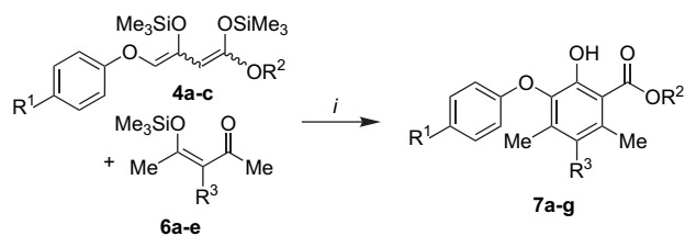
Scheme 3. Synthesis of 7a–g : (i) \text{TiCl}_4 , \text{CH}_2\text{Cl}_2 , -78 \rightarrow 20^{\circ}\text{C} , 20 h.
