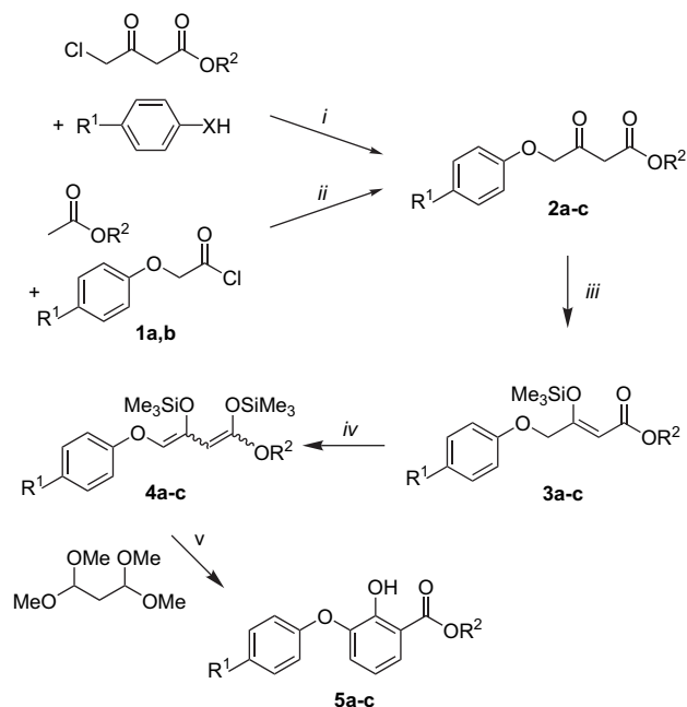
Scheme 2. Synthesis of 5a–c : (i) \text{NEt}_3/\text{KOH} , \text{CH}_2\text{Cl}_2/\text{DMSO} , 30 min, 0^{\circ}\text{C} / 5 h, 20^{\circ}\text{C} ; (ii) LDA, THF, -78 \rightarrow 20^{\circ}\text{C} , 14 h; (iii) \text{Me}_3\text{SiCl} , \text{NEt}_3 , \text{C}_6\text{H}_6 , 20^{\circ}\text{C} , 72 h; (iv) LDA, THF, -78 \rightarrow 20^{\circ}\text{C} ; (v) \text{Me}_3\text{SiOTf} , \text{CH}_2\text{Cl}_2 , -78 \rightarrow 20^{\circ}\text{C} , 20 h.
