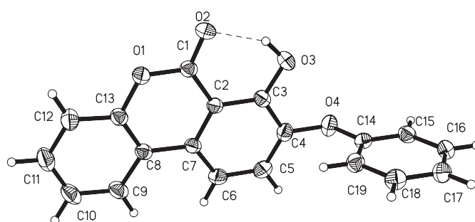
Figure 4. Ortep plot of 14 .
