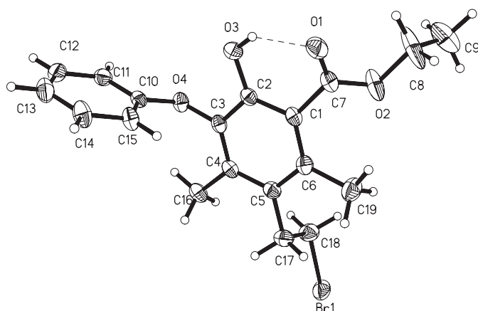
Figure 3. Ortep plot of 9b .
