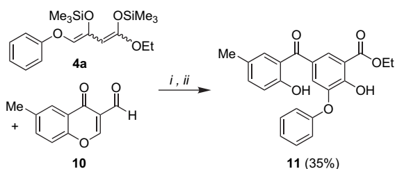
Scheme 5. Synthesis of 11 : (i) \text{Me}_3\text{SiOTf} (0.3 equiv), 20^\circ\text{C} , 10 min; (ii) (1) 4a (1.3 equiv), \text{CH}_2\text{Cl}_2 , 0 \rightarrow 20^\circ\text{C} , 12 h; (2) \text{HCl} (10%).
